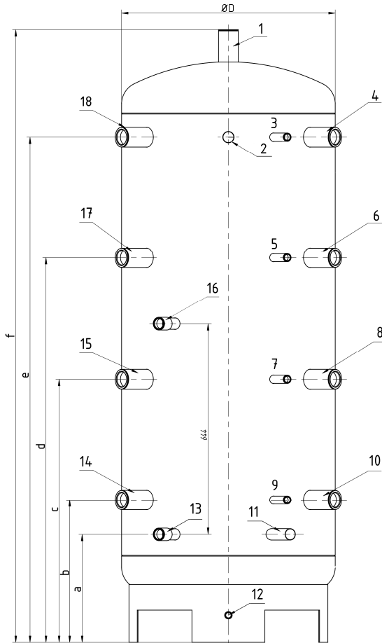
Figure 2 Sizes and connections of PT500,-750,-1000; PT500C,-750C,-1000C and PT500CF,-750CF,1000CF buffer tanks
